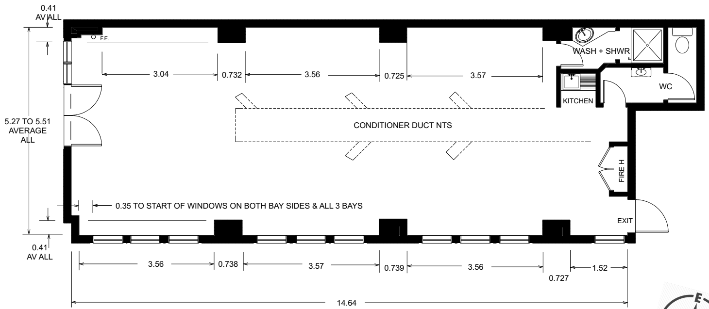
ONE LEVEL FLOOR PLAN
